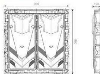
CONSTRUCTION DIAGRAM
